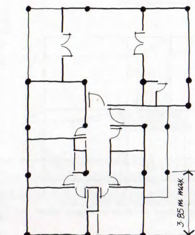
26b column layout follows partition layout
