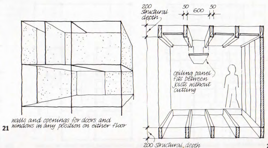
22 ceiling panel fits between joists without cutting
